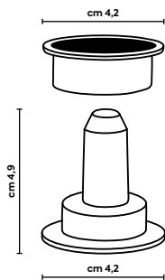
#300010 Couple conic natches
