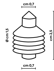
#300002 Plastic cap - big \varnothing 15 mm
