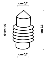
#300001 Plastic cap - medium \varnothing 10 mm
